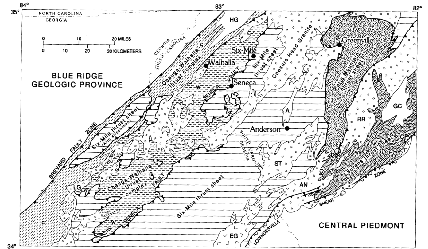
Tectonic map showing crystalline thrust sheets of the Inner Piedmont block, in northwestern South Carolina and northeastern Georgia, Modified from Nelson and others (1987). (With permission of the University of Tennessee Press).
