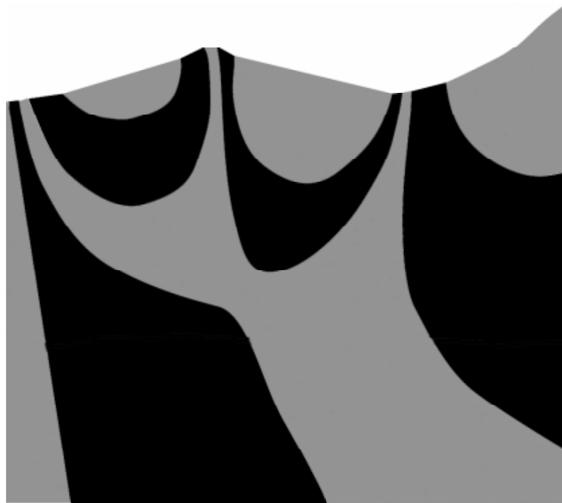
The Clemson Hydrogeology Logo was created from the above graphic which was analytically derived using Toth's (1963) Theoretical Analysis of Groundwater Flow in Small Drainage Basins.
