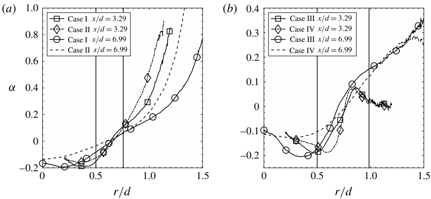
FIGURE 12. Cross-stream profiles of the segregation parameter. The downstream locations are given in the legend.
