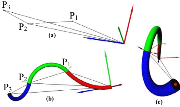
Fig. 7 – Results of the algorithms in section III.A and IV.B. Graphic (a) illustrates the result of IV.B exhibiting the orientation of triangles \triangle Op_2p_3 and \triangle Op_1p_2 in 3-D space. \triangle Op_2p_3 and \triangle Op_1p_2 lie in two different planes in space inclined at an angle to each other. The angles of orientation of the triangular planes are termed dihedral angles. Items (b) and (c) illustrate a continuum trunk fit to the skeleton in (a) from differing perspectives.
