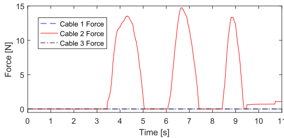
(b) Generated forces corresponding to bending of distal section with known planar obstacle.
