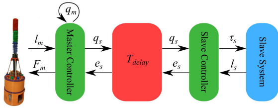
Fig. 5. Teleoperation scheme for HaptOct.
