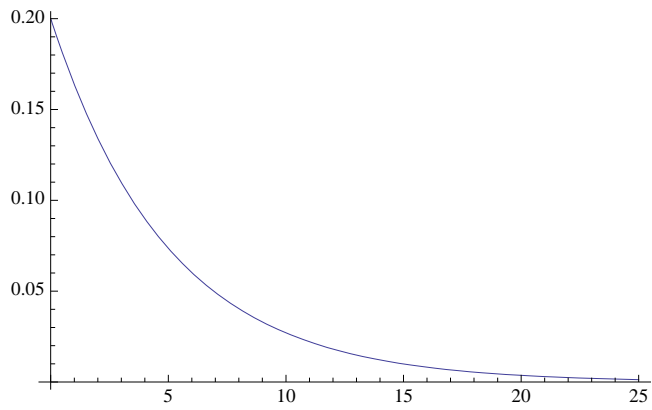
Gamma with parameters \alpha = 1, \lambda = 0.2
