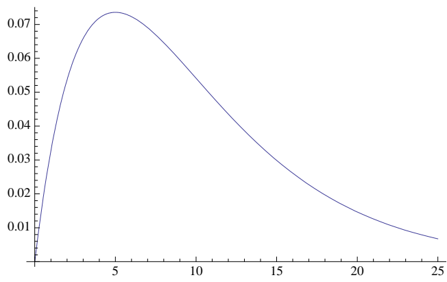
Gamma with parameters \alpha = 2, \lambda = 0.2
