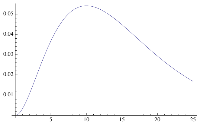
Gamma with parameters \alpha = 3, \lambda = 0.2
