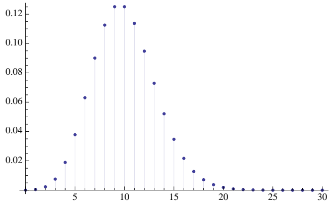
Poisson with \lambda = 10
