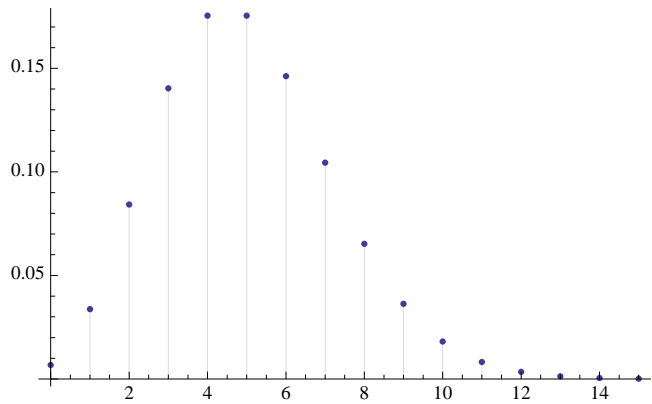
Poisson with \lambda = 5
