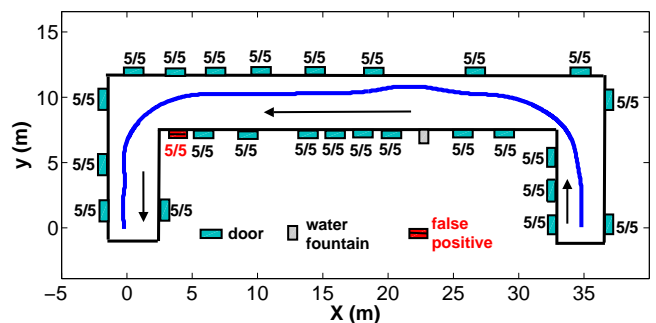
Fig. 17. TOP: Two images of the hallway environment near our laboratory. BOTTOM: 2D plan view of the hallway, along with the results of the experiment. Beside each door is indicated the number of detections / total number of trials.
